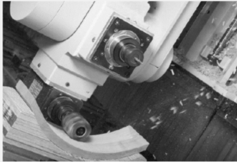
Eight 5 Axis CNC: Chair parts design and production
